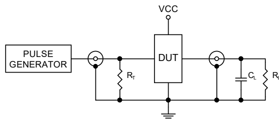
Figure4. Test Circuit
