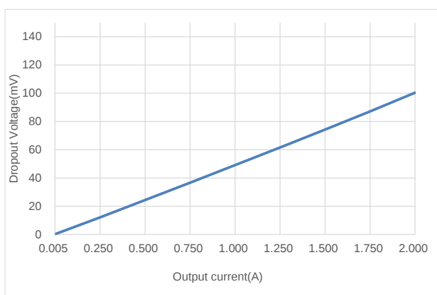
Drop Voltage VS Output Current
