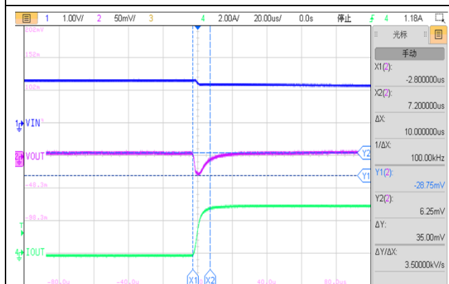
Load Transient Response V_{IN}=1.1V , V_{BIAS}=3V , V_{OUT}=0.8V , I_{OUT}=1mA\sim 3000mA
