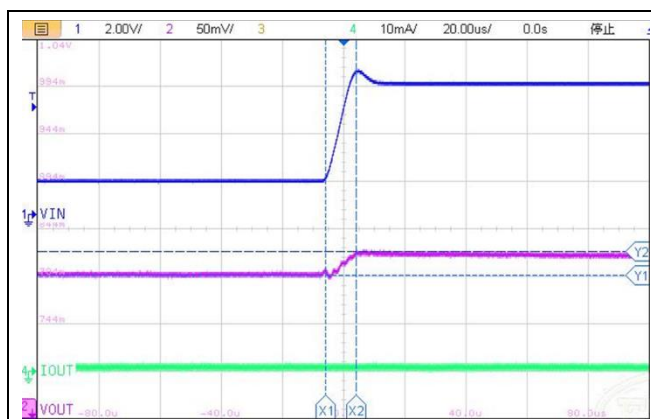
Line Transient Response V_{IN}=1.4V\sim 5.5V , V_{OUT}=0.8V , I_{OUT}=1mA
