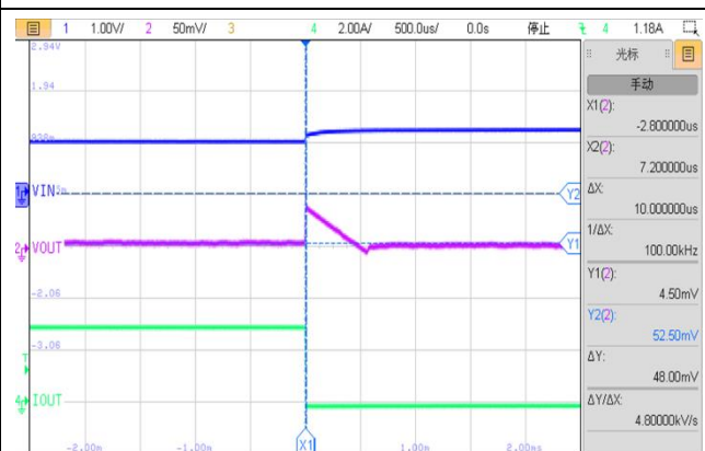
Load Transient Response V_{IN}=1.1V , V_{BIAS}=3V , V_{OUT}=0.8V , I_{OUT}=3000mA\sim 1mA
