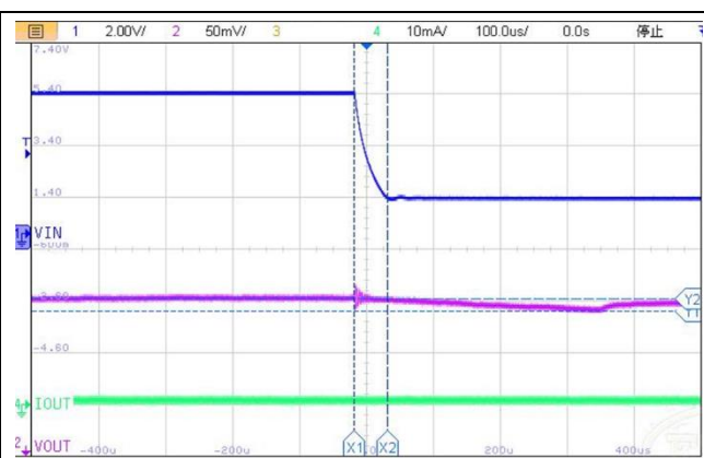
Line Transient Response V_{IN}=5.5V\sim 1.4V , V_{OUT}=0.8V , I_{OUT}=1mA
