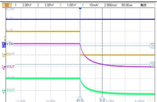
PSRR @ 30mA
