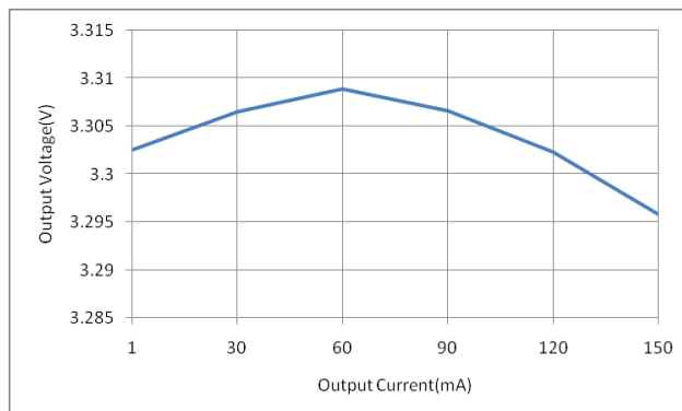
Output Voltage VS Output Current(V IN =8V)
