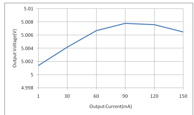
Output Voltage VS Output Current( V_{IN}=7V )
