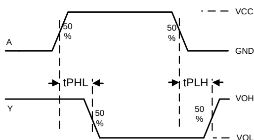
Figure 3. Switching Waveform
