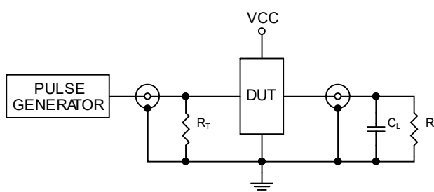
Figure4. Test Circuit
