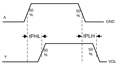
Figure 3. Switching Waveform
