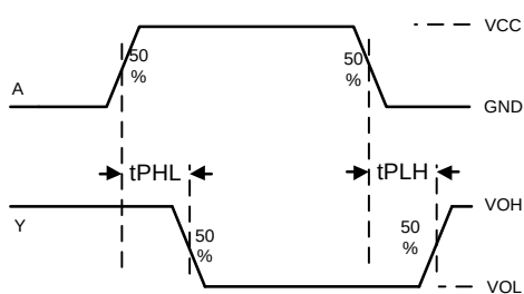
Figure 3. Switching Waveform
