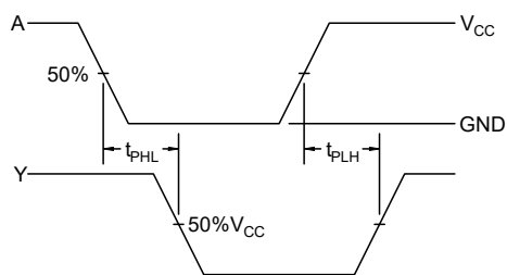
Figure 3. Switching Waveforms
