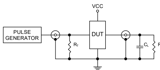
Figure 4. Test Circuit
