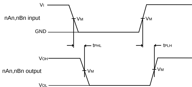
Fig.5 The data input (nAn, nBn) to output (nBn, nAn) propagation delay times
