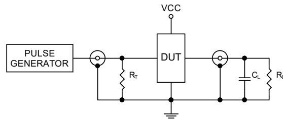
Figure4. Test Circuit
