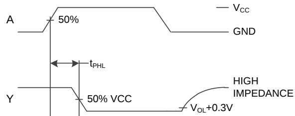
Figure3. Switching Waveforms
