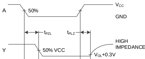
Figure 3. Switching Waveform
