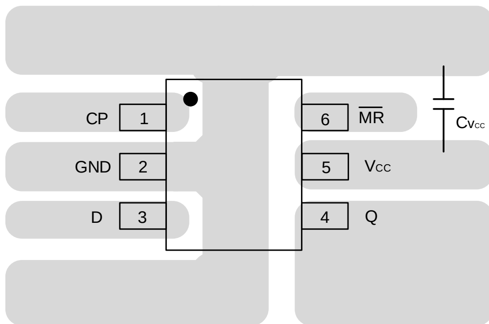
Fig.7 Layout Guide
