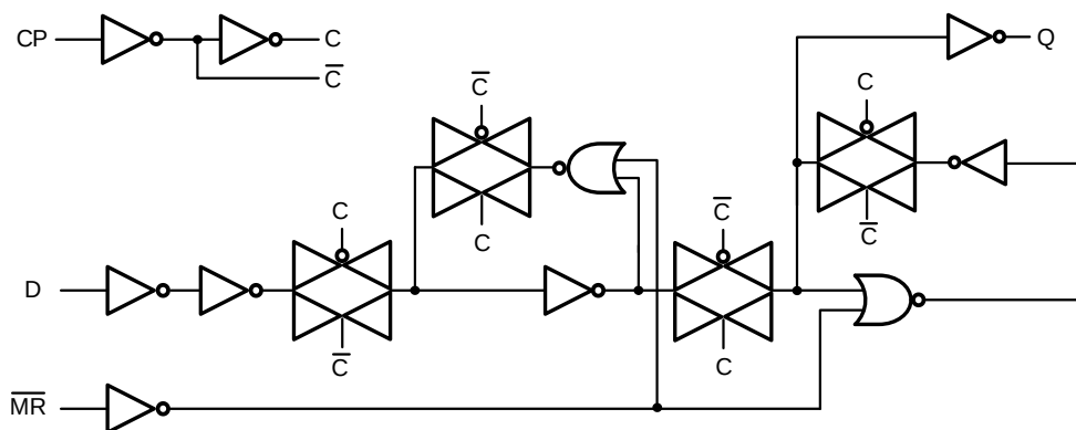
Fig 3. Logic Diagram
