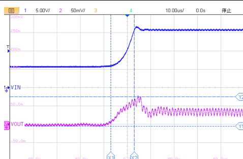
10us/div, V_{OUT}=5.0V I_{OUT} = 1A V_{IN}=6.5V to 17V Figure39. ET8123 Line Transient
