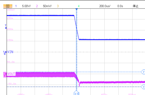
200us/div, V_{OUT}=5.0V I_{OUT} = 1A V_{IN}=17V to 6.5V Figure40. ET8123 Line Transient
