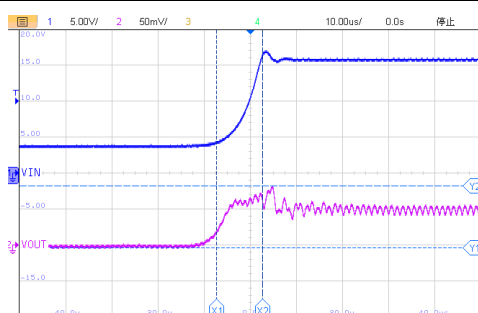
10us/div, V_{OUT}=3.3V I_{OUT} = 1A V_{IN}=4.5V to 17V Figure37. ET8123 Line Transient
