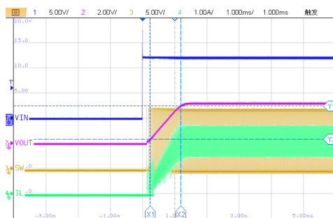
1ms/div, V_{EN}=5V V_{OUT}=3.3V I_{OUT}=2A Figure45. ET8123 Start-Up Relative to V_{IN}
