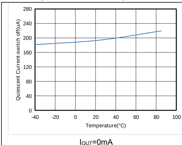
Figure1. ET8123 Quiescent current vs Temperature
