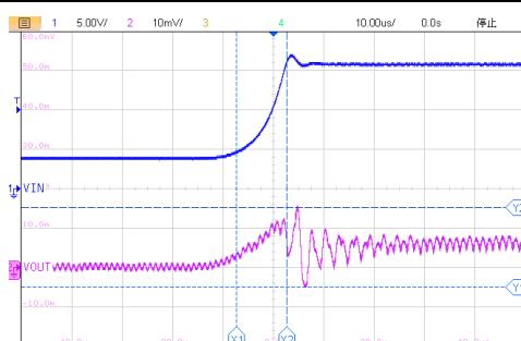
5us/div, V_{OUT}=1.0V I_{OUT} = 1A V_{IN}=4.5V to 17V Figure35. ET8123 Line Transient
