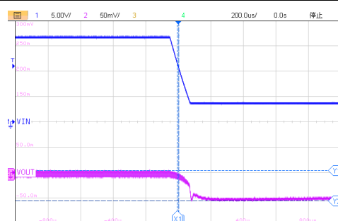
200us/div, V_{OUT}=3.3V I_{OUT} = 1A V_{IN}=17V to 4.5V Figure38. ET8123 Line Transient
