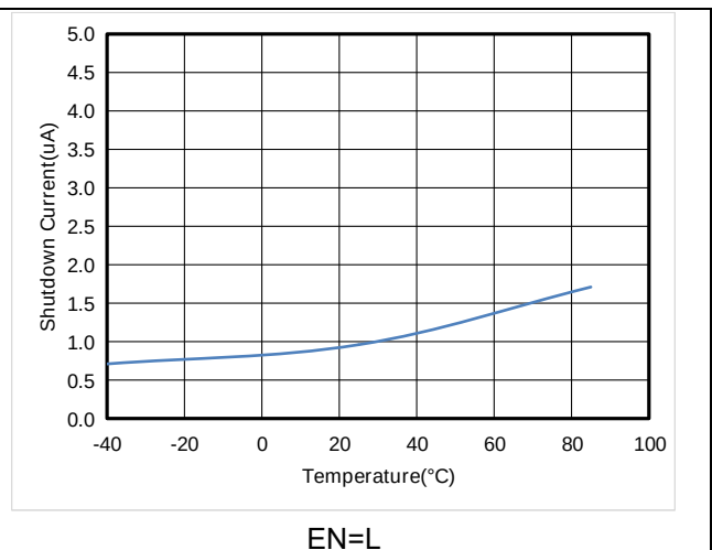
Figure2. ET8123 Shutdown current vs Temperature
