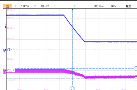
200us/div, V_{OUT}=1.0V I_{OUT} = 1A V_{IN}=17V to 4.5V Figure36. ET8123 Line Transient
