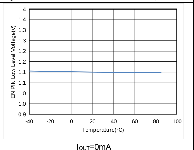
Figure4. ET8123 EN_L vs Temperature
