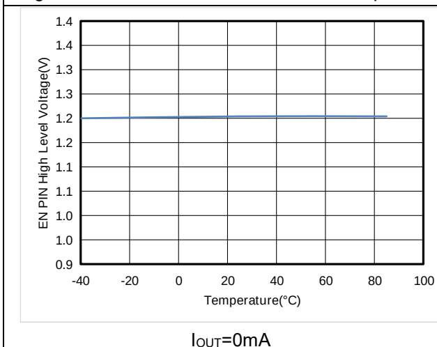
Figure3. ET8123 EN_H vs Temperature
