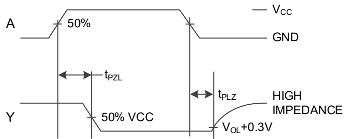
Figure3. Switching Waveforms
