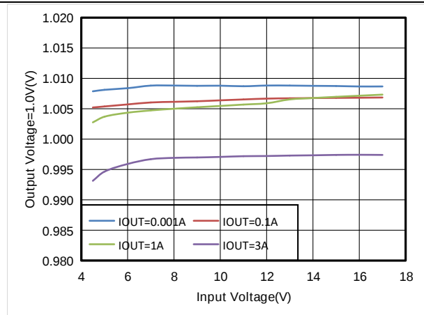
Figure14. ET81311 Line Regulation, V_{OUT}=1.0V
