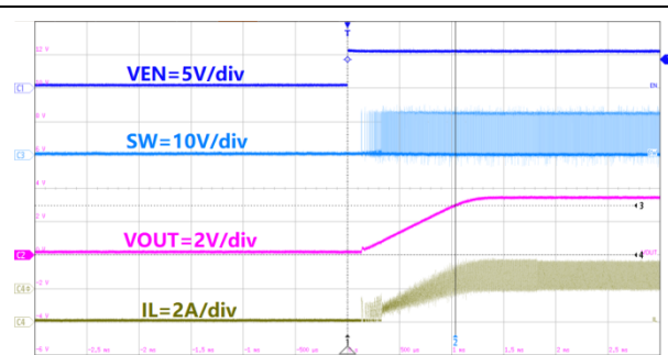
Figure42. ET81311 Start-Up Relative to EN
