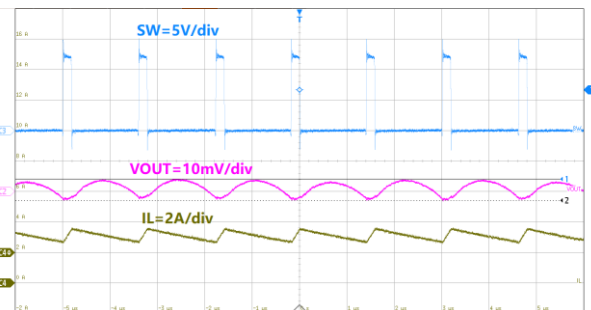
1us/div, V_{OUT}=1.0V I_{OUT}=3A Figure20. ET81311 Output Ripple
