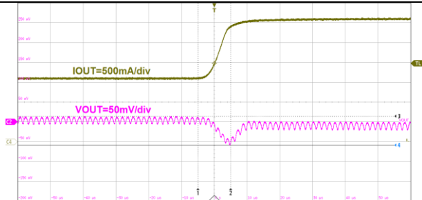
10us/div, V_{OUT}=3.3V I_{OUT} = 1.5A to 3A Figure31. ET81311 Load Transient
