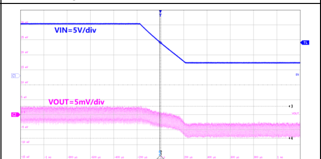
200us/div, V_{OUT}=1.0V I_{OUT} = 1.5A V_{IN}=17V to 4.5V Figure36. ET81311 Line Transient
