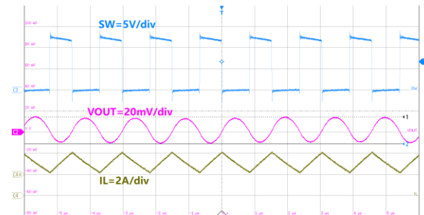
1us/div, V_{OUT}=5.0V I_{OUT}=3A Figure28. ET81311 Output Ripple
