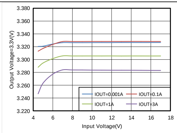
Figure15. ET81311 Line Regulation, V_{OUT}=3.3V
