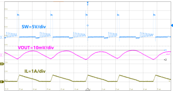
1us/div, V_{OUT}=1.0V I_{OUT}=250mA Figure18. ET81311 Output Ripple
