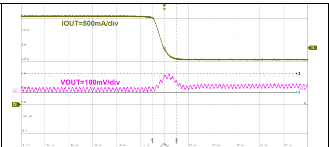
10us/div, V_{OUT}=5.0V I_{OUT} = 3A to 1.5A Figure34. ET81311 Load Transient
