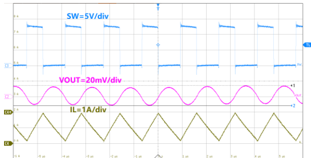
1us/div, V_{OUT}=5.0V , I_{OUT}=1A Figure27. ET81311 Output Ripple
