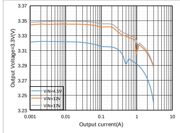
Figure12. ET81311 Load Regulation, V_{OUT}=3.3V
