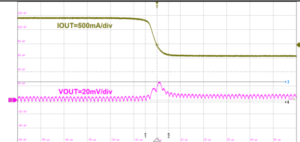
10us/div, V_{OUT}=1.0V I_{OUT} = 3A to 1.5A Figure30. ET81311 Load Transient
