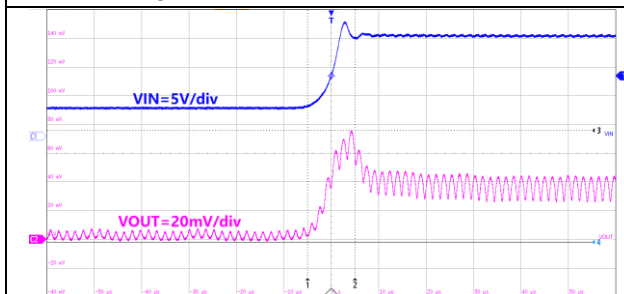
10us/div, V_{OUT}=3.3V I_{OUT} = 1.5A V_{IN}=4.5V to 17V Figure37. ET81311 Line Transient
