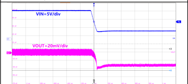
200us/div, V_{OUT}=3.3V I_{OUT} = 1.5A V_{IN}=17V to 4.5V Figure38. ET81311 Line Transient
