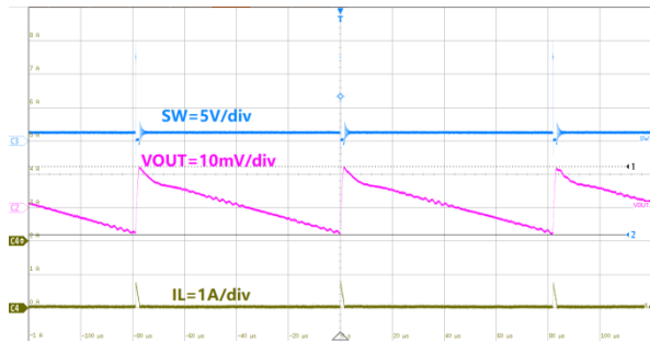
20us/div, V_{OUT}=1.0V I_{OUT}=10mA Figure17. ET81311 Output Ripple
