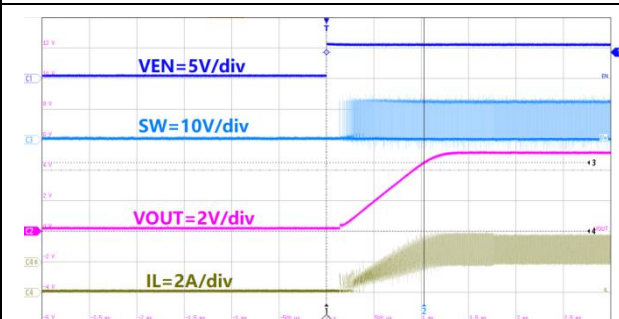
Figure41. ET81311 Start-Up Relative to EN
