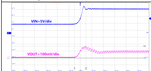
10us/div, V_{OUT}=5.0V I_{OUT} = 1.5A V_{IN}=6.5V to 17V Figure39. ET81311 Line Transient
