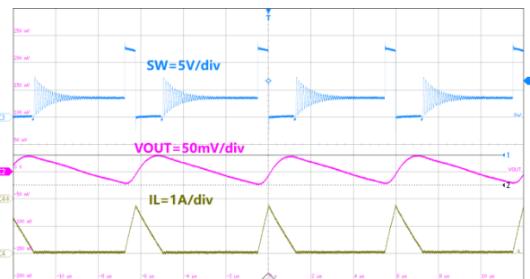
2us/div, V_{OUT}=3.3V I_{OUT}=250mA Figure22. ET81311 Output Ripple
