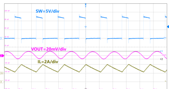
1us/div, V_{OUT}=3.3V I_{OUT}=3A Figure24. ET81311 Output Ripple
