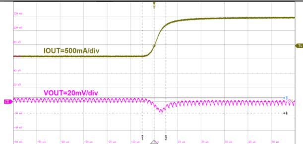
10us/div, V_{OUT}=1.0V I_{OUT} = 1.5A to 3A Figure29. ET81311 Load Transient
