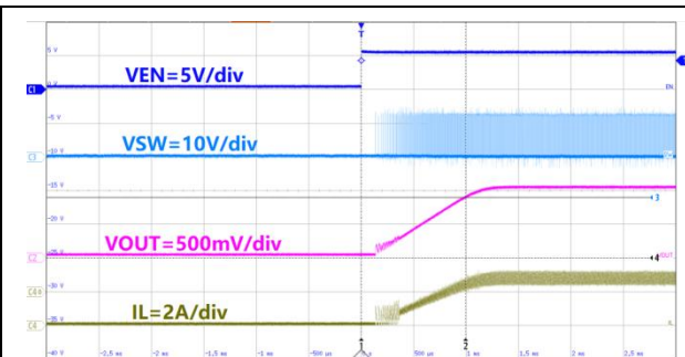
Figure41. ET81311 Start-Up Relative to EN
