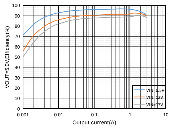
Figure8. ET81311 Efficiency vs Output Current
