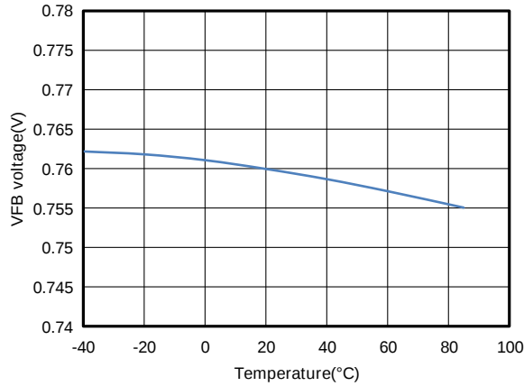
Figure5. ET81311 VFB Voltage vs Temperature
