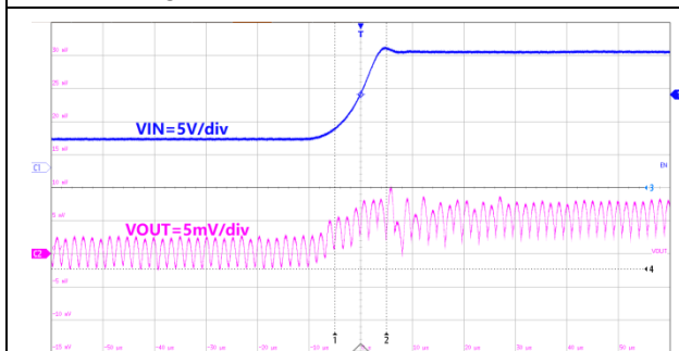
10us/div, V_{OUT}=1.0V I_{OUT} = 1.5A V_{IN}=4.5V to 17V Figure35. ET81311 Line Transient
