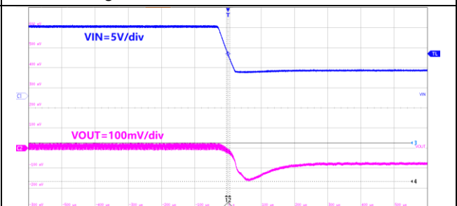
200us/div, V_{OUT}=5.0V I_{OUT} = 1.5A V_{IN}=17V to 6.5V Figure40. ET81311 Line Transient
