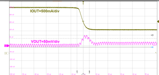
10us/div, V_{OUT}=3.3V I_{OUT} = 3A to 1.5A Figure32. ET81311 Load Transient
