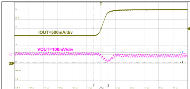
10us/div, V_{OUT}=5.0V I_{OUT} = 1.5A to 3A Figure33. ET81311 Load Transient
