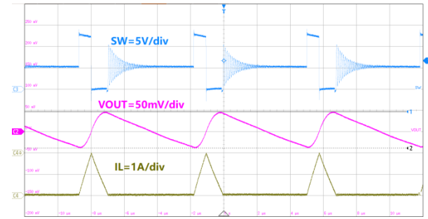
2us/div, V_{OUT}=5.0V I_{OUT}=250mA Figure26. ET81311 Output Ripple
