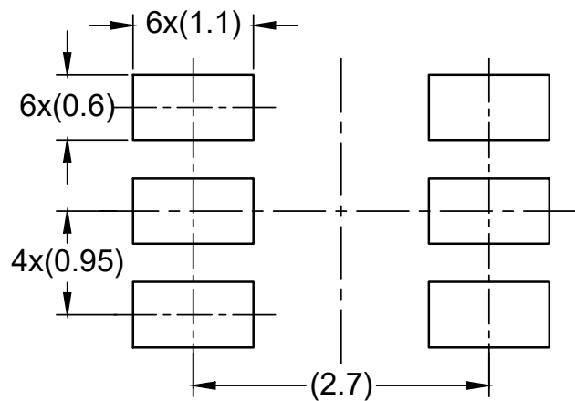
LAND PATTERN EXAMPLE
