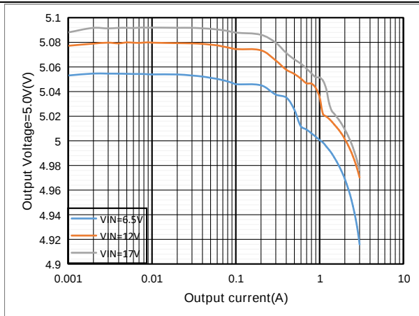
Figure13. ET81311 Load Regulation, V_{OUT}=5.0V
