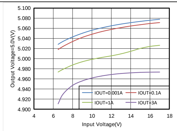
Figure16. ET81311 Line Regulation, V_{OUT}=5.0V
