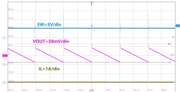
100us/div, V_{OUT}=5.0V I_{OUT}=10mA Figure25. ET81311 Output Ripple
