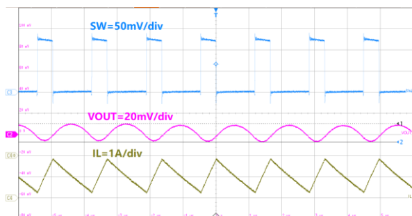
1us/div, V_{OUT}=3.3V I_{OUT}=1A Figure23. ET81311 Output Ripple
