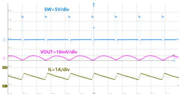
1us/div, V_{OUT}=1.0V I_{OUT}=1A Figure19. ET81311 Output Ripple
