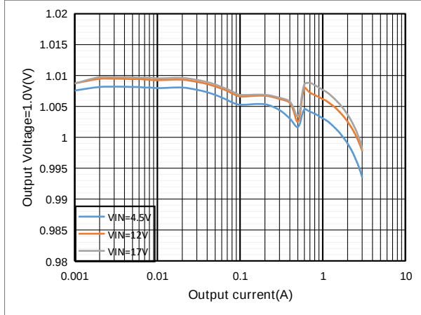
Figure11. ET81311 Load Regulation, V_{OUT}=1.0V
