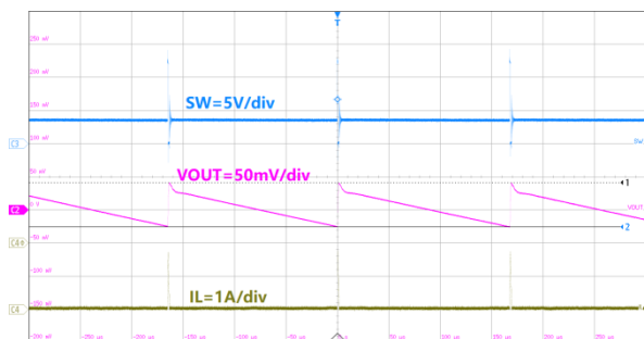
50us/div, V_{OUT}=3.3V I_{OUT}=10mA Figure21. ET81311 Output Ripple
